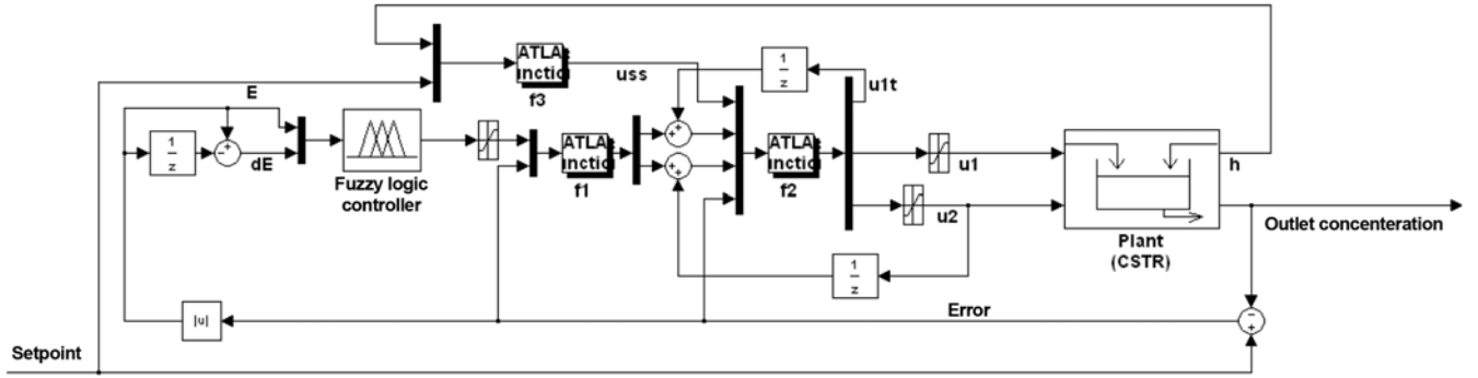
Fig. 12. Control circuit.
